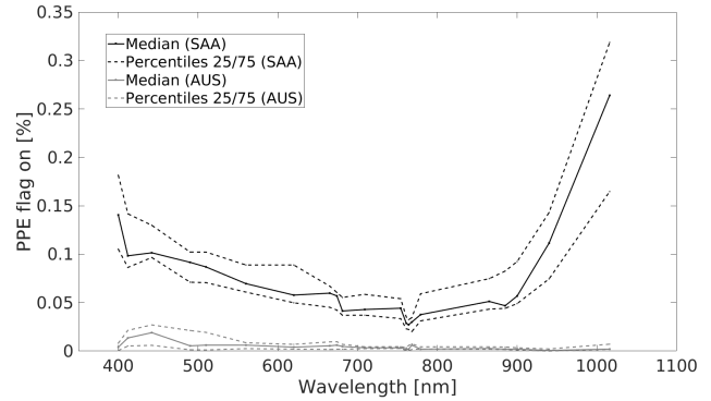
Fig. 6. Percentage of pixels flagged as PPE contaminated, evaluated over a set of 18 subsets of 1 squared degree, 9 from each region, SAA (black curves) and AUS (gray curves). The amount of affected pixels is on average 27.8 times larger in the SAA region, although the difference is higher at the spectral extremes [Oa_01 (400 nm) and Oa_21 (1016 nm) bands].
