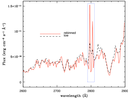
Fig. 3. IUE low-dispersion (dashed line) and rebinned (solid line) spectra of HD 22 049, both observed on January, 14th 1984 with a time difference of 1 h.
