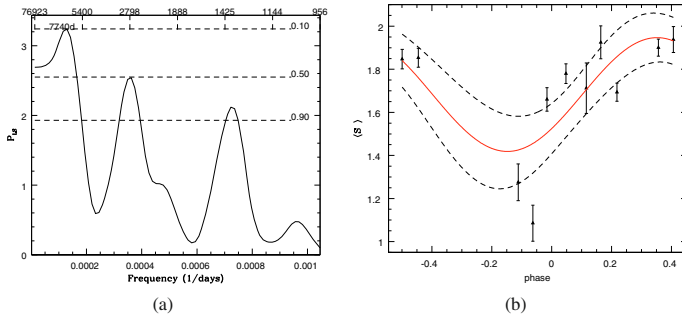
Fig. 14. HD 224 085 – II Peg. Left: Lomb-Scargle periodogram of the mean annual \langle S \rangle of the data plotted in Fig. 13. The False Alarm Probability (FAP) levels of 10, 50 and 90% are indicated. Right: the mean annual \langle S \rangle of the data plotted in Fig. 13 phased with the period of 7740 \pm 207 days ( 21.21 \pm years 0.57 ). The solid line shows the harmonic curve that best fits the observations and the dashed lines indicate the points that apart \sigma from that fit.
