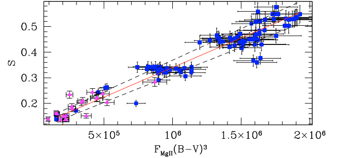
Fig. 1. S vs. F_{\text{MgII}}(B - V)^3 for the set of 117 nearly simultaneous observations of Mount Wilson index and IUE high-resolution Mg II h and k fluxes for dwarfs we used in Paper I (■). We considered errors of 10% for F_{\text{MgII}} and 6% for S . The least square fit (solid line) has a correlation coefficient of 0.95. The dotted lines indicate \pm 3\sigma from the fit. The triangles (▲) represent non-simultaneous Mount Wilson indices and IUE high-resolution Mg II fluxes of cool sub-giant stars, not used in the calibration.
