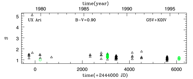
Fig. 10. HD 21 242 – UX Ari. Symbols as in Fig. 6.
