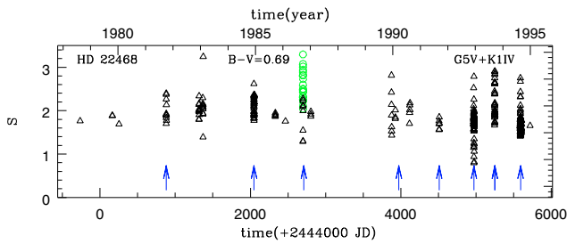
Fig. 6. HD 22468 – V711 Tau – HR 1099. We indicate the Mount Wilson index S obtained from the IUE high and low-resolution spectra with triangles ( \Delta ) and circles ( \circ ) respectively. We indicate with arrows the sets of data for which we analysed the short-term variability.
