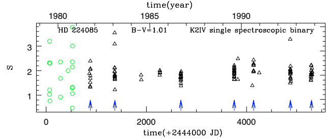
Fig. 13. HD 224 085 – II Peg. Symbols as in Fig. 6.
