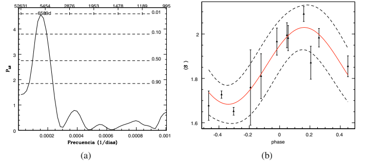
Fig. 8. HD 22468 – V711 Tau – HR 1099. Left: Lomb-Scargle periodogram of the mean annual \langle S \rangle of the data plotted in Fig. 6. The False Alarm Probability (FAP) levels of 1, 10, 50 and 90% are indicated. Right: the mean annual \langle S \rangle of the data plotted in Fig. 6 phased with the period of 6589 days. The solid line shows the harmonic curve that best fits the data with a reduced \chi^2 = 1.5 and the dashed lines indicate the points that apart \sigma from that fit.
