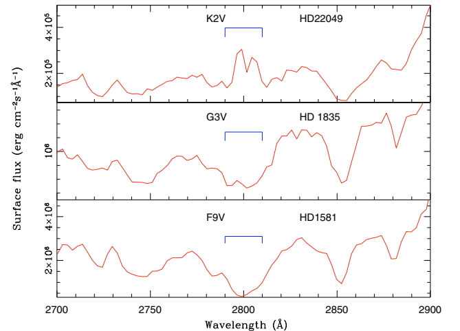
Fig. 2. IUE low-resolution spectra of three representative stars: HD 22 049 (K2V), HD 1835 (G3V) and HD 1581 (F9V). Surface flux is obtained according to Eq. (1). The windows used to integrate the line-core emission (2790–2810 Å) are marked on each spectrum.
