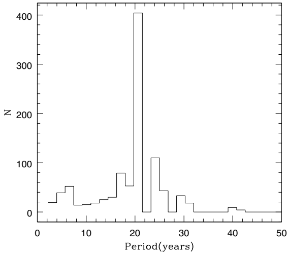
Fig. 12. Histogram of the detected periods (with maximum significance) for sample of 1000 different sets the sunspot number re-scaled to 25 years.
