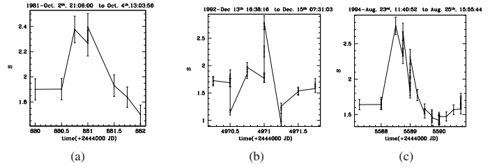
Fig. 7. HD 22468 – V711 Tau – HR 1099. Three flares on 1981, Oct. 3rd; 1992, Dec. 14th and 1994, Aug. 24th.
