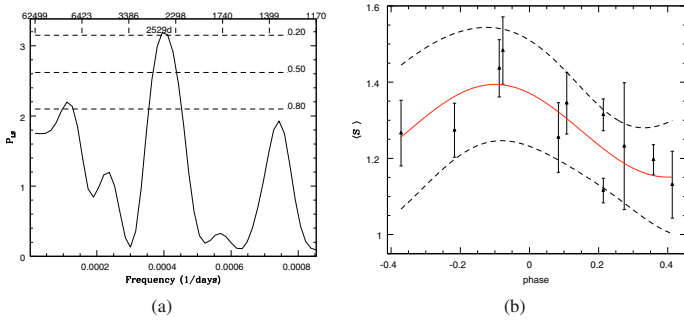
Fig. 11. HD 21 242 - UX Ari. Left: Lomb-Scargle periodogram of the mean annual \langle S \rangle of the data plotted in Fig. 10. The False Alarm Probability (FAP) levels of 20, 50 and 80% are indicated. Right: the mean annual \langle S \rangle of the data plotted in Fig. 10 phased with the period of 2529 \pm 101 days ( 6.95 \pm 0.5 years). The solid line shows the harmonic curve that best fits the data with a reduced \chi^2 = 3 and the dashed lines indicate the points that apart \sigma from that fit.
