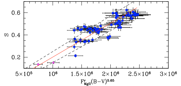
Fig. 4. S vs. F_{\text{MgII}}^r (B - V)^{5.65} for the stars listed in Table 1. We considered errors of 10% for F_{\text{MgII}}^r and 6% for S . The least square fit (solid line) has a correlation coefficient of 0.82. The dotted lines indicate the points that apart \pm\sigma from the fit. The triangles (▲) represent non-simultaneous Mount Wilson indices and IUE high-resolution Mg II fluxes of cool sub-giant stars with B - V > 0.65 , not used in the calibration.
