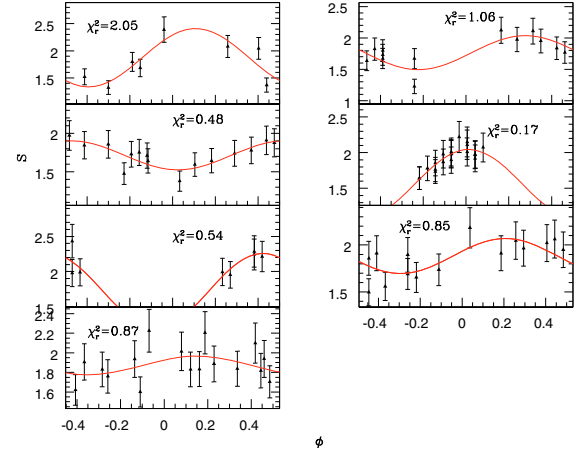
Fig. 16. Variability on HD 224 085- II Peg. Light curves S vs. \phi of the datasets indicated with arrows in Fig. 13. We plotted the harmonic curve that best fit the data, the number in each plot refers to reduced \chi^2 of the fit.
