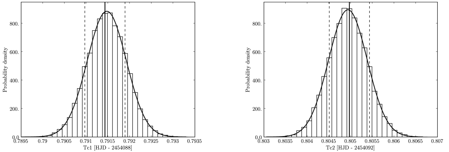
Fig. 2.—Probability density distributions for the central times of the transits obtained from the MCMC simulations. The thick vertical solid line indicates the median of the distribution, and the dotted lines mark the upper and lower 68% confidence limits. The solid (blue) curve is a Gaussian distribution with the same mean and standard deviation as the data. [See the electronic edition of the Journal for a color version of this figure.]
