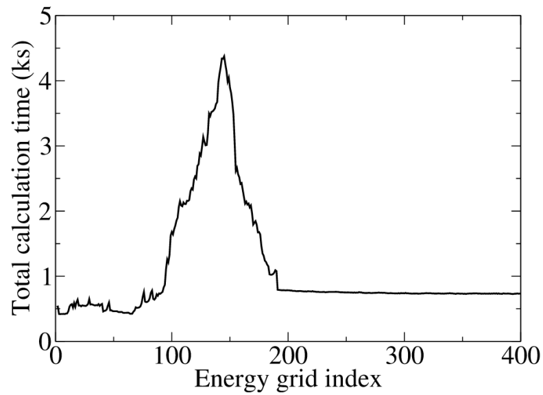
Fig. 3. Total processor time spent in each energy \text{Ni}^{3+} . The calculation of the transition matrix S turns much slower when the number of open channels n_o and closed channels n_c is similar.
