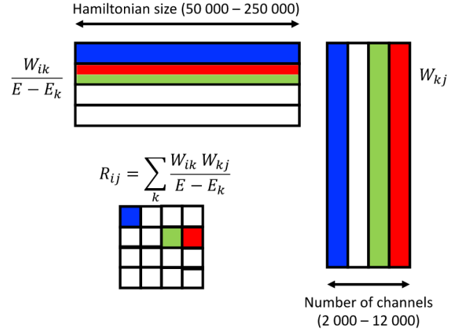
Fig. 2. Half of the symmetric R-matrix is calculated by 10 matrix multiplications, and then symmetrised for the full result. We optimise the memory usage of the GPU, by allowing several MPI tasks to access the GPU simultaneously. In the figure, the blue, red and green blocks are representative of a particular task of matrix multiplication sent to the GPU, three in present case. In general, each task calculates in a different energy and partial wave, and hence the submatrix of a different R-matrix. (For interpretation of the references to color in this figure legend, the reader is referred to the web version of this article.)
