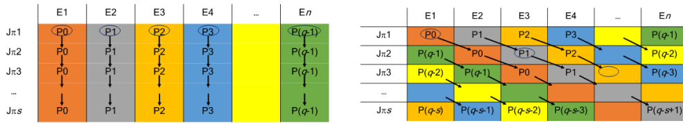
Fig. 1. Diagram of energies and symmetries worked by each processor. Left: v0.87; right v1.1. P_i represents the processor, it is also represented by a particular color; E_i represents the energy array to be processed by processor P_i in the partial wave J\pi . The oval represents the partial wave where the processor P_i starts calculating. (For interpretation of the references to color in this figure legend, the reader is referred to the web version of this article.)
