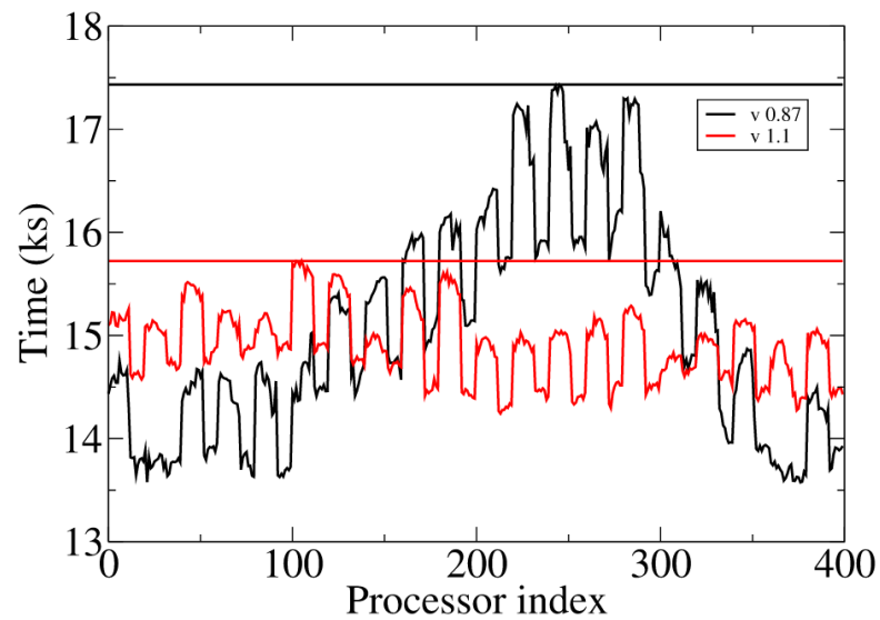
Fig. 4. Total time of each processor \text{Ni}^{3+} . The horizontal lines mark the total calculation time (maximum).
