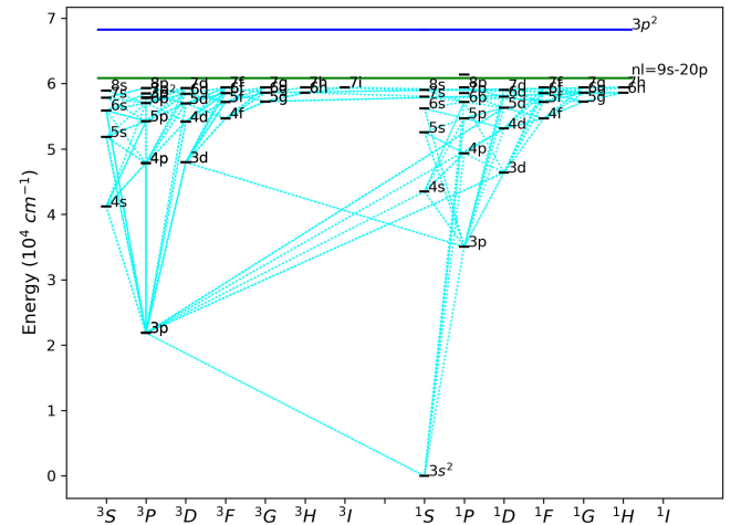
Fig. 4. Mg I Grotrian diagram for the structure of 85-level models. Fine structure is included up to level 7i^1I (level 54, 59 430.517 cm -1 ) (not distinguishable in the figure). The first 54 energy levels are fully represented. Superlevels (between nl=9s and 20p ) are shown with their average energy as a solid green line, very close to the continuum (which occurs at 61 671.05 cm -1 ). Level 3p^2 (68 275 cm -1 ) is represented as a solid blue line. In cyan dashed lines, the 210 transitions included in the spectrum are shown.
