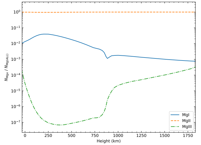
Fig. 3. Mg I (blue line), Mg II (orange dashed line), and Mg III (green dash-dotted line) densities relative to the total magnesium density for atmospheric model 1401 as a function of height.
