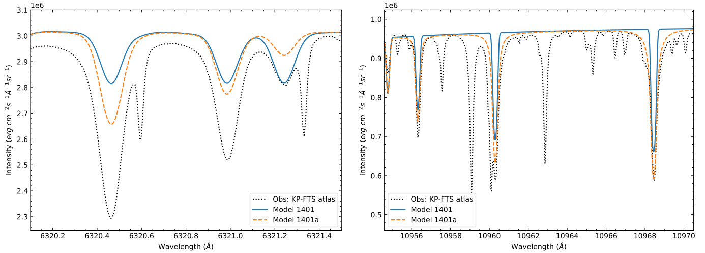
Fig. 7. Models 1401 (blue line) and 1401a (orange dashed line) compared to Kitt Peak Solar Atlas (KP-FTS) (Hase et al. 2010) intensity observations (black dashed line). Triplet transition around 6320 Å ( left panel ) shows improvements due to the update to the oscillator strength parameters, and the 10964.38 Å profile ( right panel ) shows improvements due to changes in the broadening data (not included in model 1401).
