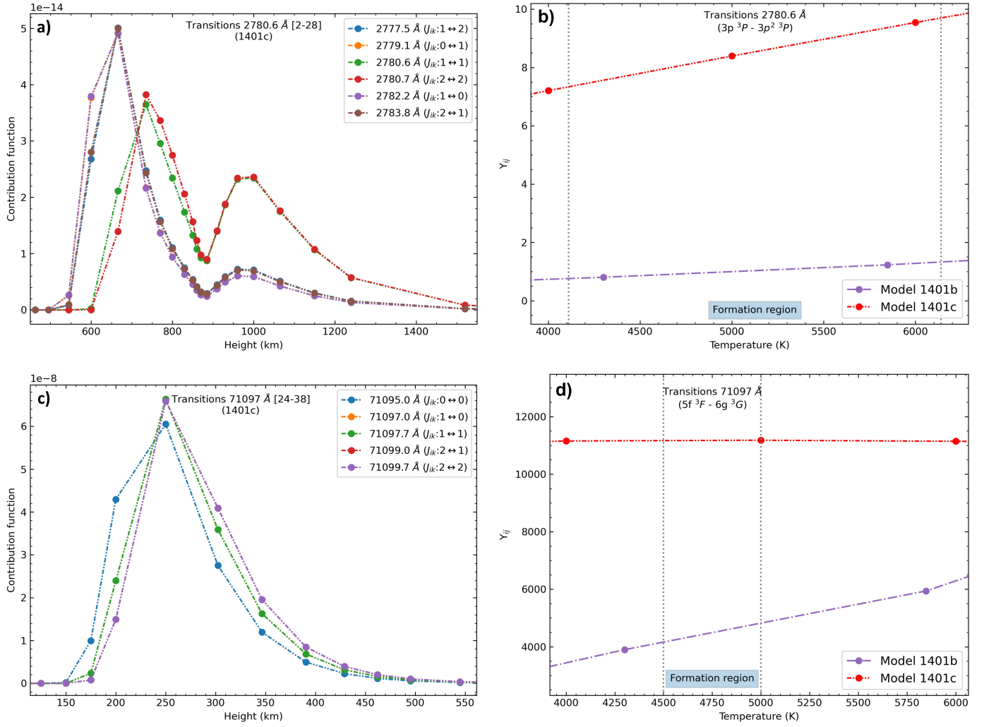
Fig. 14. Left panel (a and c): 1401c model contribution functions through the atmospheric height for lines involved in transitions 2780.6 Å (a) and 71097 Å (c). Right panel (b and d): effective collision strength ( \Upsilon_{ij} ) data at the formation region temperatures that were used to compute the populations for 2780.6 Å (b) and 71097 Å (d) transitions in models 1401b (purple dashed-dotted line) and 1401c (red dashed-double-dotted line). The \Upsilon_{ij} data provided by the DW method are greater than the SEA&VRM for all the transitions studied.
