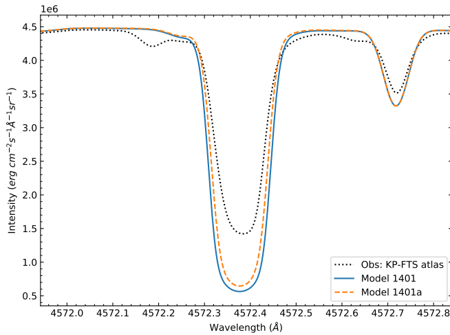
Fig. 6. Models 1401 (blue line) and 1401a (orange dashed line) compared to Kitt Peak Solar Atlas (KP-FTS) (Hase et al. 2010) intensity observations (black dotted line). Transition 4572.4 Å shows a small improvement due to an update to the oscillator strength parameter, whose value decreased by 41%.
