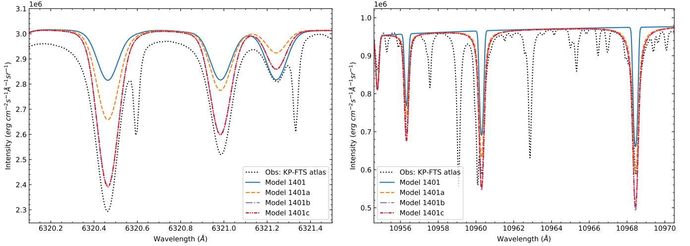
Fig. 10. VIS and NIR spectral lines. Models 1401 (blue line), 1401a (orange dashed line), 1401b (purple dashed-dotted line), and 1401c (red dashed-double-dotted line) vs. observations (black dotted line). Left. Visible range: transitions 6320.72 Å compared to Kitt Peak Solar Atlas (KP-FTS) (Hase et al. 2010) intensity observations. Changes due to a higher number of levels (models 1401b and 1401c) are clearly visible. Right. NIR range: transitions 10964.38 Å show improvements due to changes in the broadening data (not included in model 1401) and the increment in the number of energy levels (models 1401b and 1401c).
