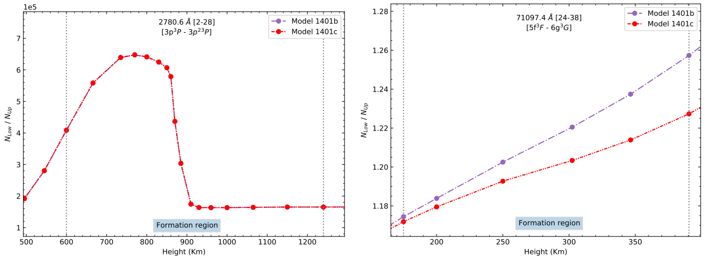
Fig. 15. Level Population ratio ( N_{low}/N_{up} ) at formation heights for transitions 2780.6 Å (left) and 71097 Å (right), following the examples in Figs. 14a and b and Figs. 14c and d, respectively. Left panel: the ratios are identical for models 1401b (purple dashed-dotted line) and 1401c (red dashed-double-dotted line), producing the same line (shown in Fig. 9). Right panel: as in almost every IR transition, level population ratios are higher in model 1401b, producing deeper spectral lines (the line for this example is shown in Fig. 11d).
