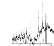
FIG. 1. Experimental spectrum of Fe in laser-produced plasma (this work), compared with theoretical data. The intensity of each array was adjusted to obtain the best fit. 3d^5 4s^1 4p transitions: 4.3 \rightarrow 4d^5 4s^1 4p , 4.3 \rightarrow 4d^5 4s^1 4p , 4.3 \rightarrow 4d^5 4s^1 4p , 4.3 \rightarrow 4d^5 4s^1 4p , 4.3 \rightarrow 4d^5 4s^1 4p , 4.3 \rightarrow 4d^5 4s^1 4p , 4.3 \rightarrow 4d^5 4s^1 4p , 4.3 \rightarrow 4d^5 4s^1 4p , 4.3 \rightarrow 4d^5 4s^1 4p , 4.3 \rightarrow 4d^5 4s^1 4p .
